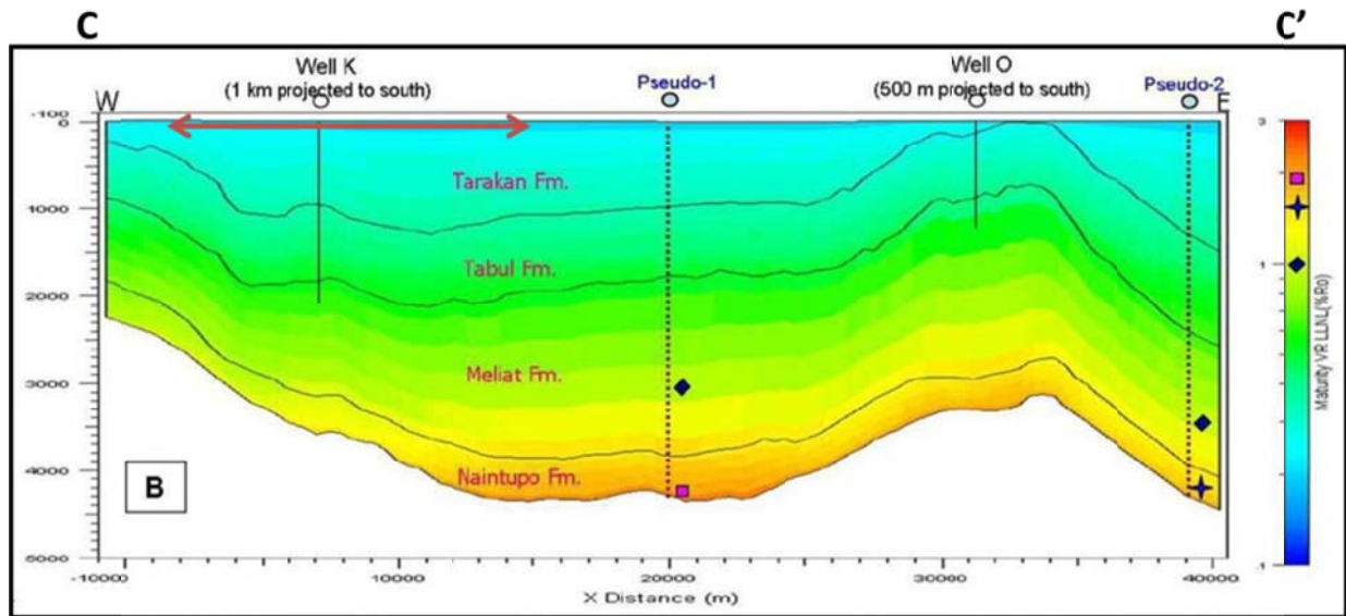
Figure XXIII-9. West-East Trending Structural Cross-section Across the Onshore North-Central Tarakan Basin, Showing Generally Simple Structural Conditions. Source Rocks of the Tabul Formation Occur at Prospective Depths of 1 to 2 Km with Oil-prone R_o of 0.6% to 0.7%. Vertical Exaggeration = 3x.
